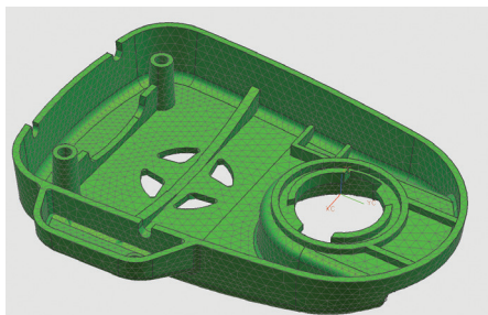
Initial analysis model.
