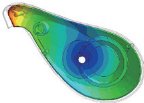
3D Warpage Prediction
