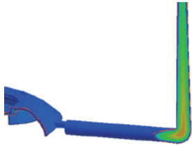
3D Runner Modeling
